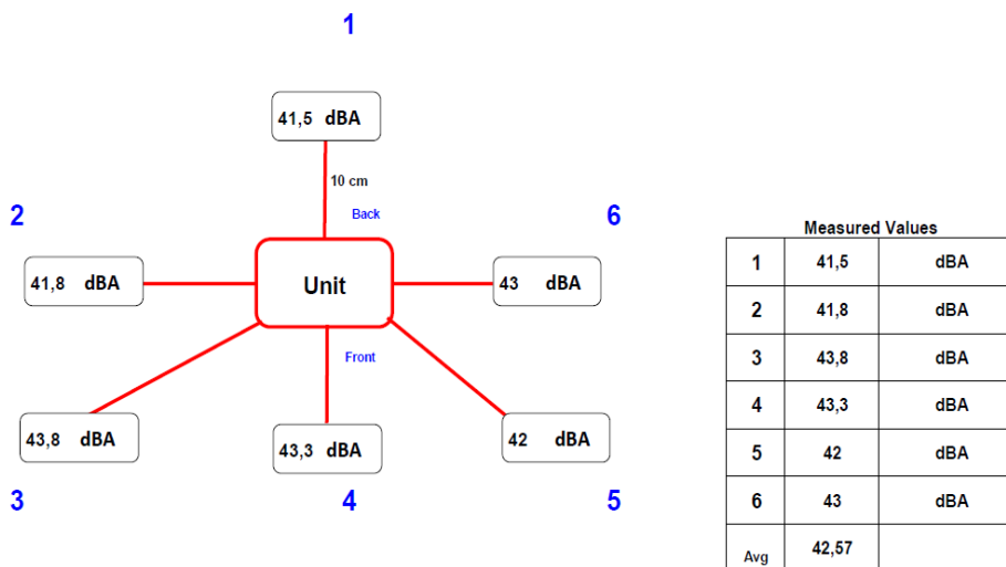
Figure 8: MJF Sound-Noise Level Test
