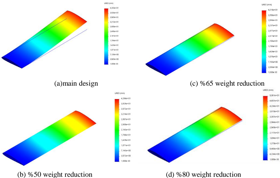
Figure 3. Total deformation values as a result of Solidworks structural analysis
