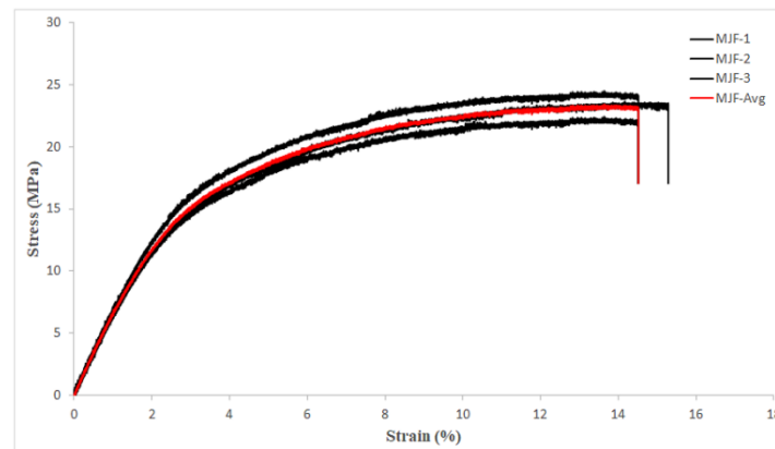
Figure 5: MJF Tensile Stress- Strain Graph
