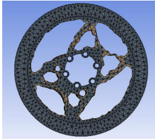
Figure 4. Lightened disc rotor as a result of topological optimization
