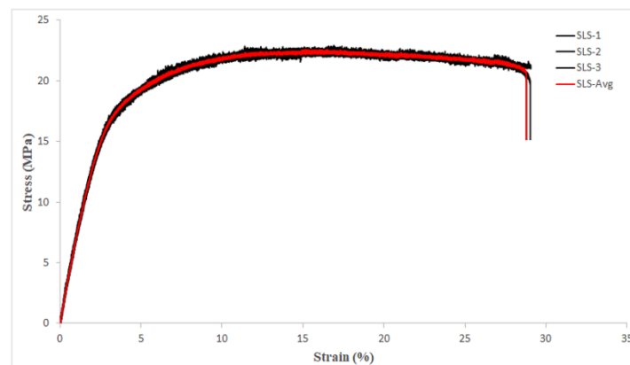
Figure 6: SLS Tensile Stress- Strain Graph
