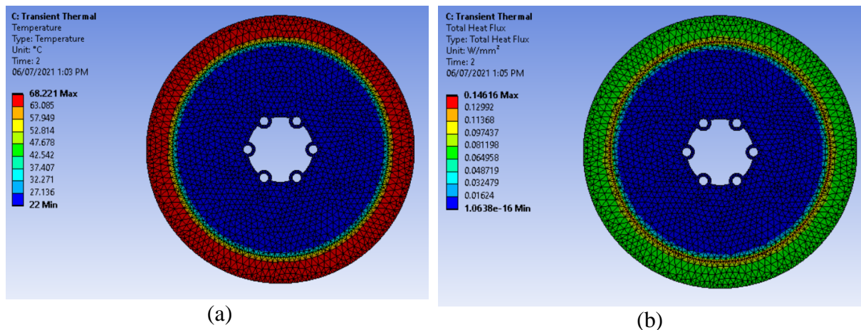
Figure 3. Rotor (a) temperature (°C) and (b) heat flux distribution (W/mm 2 ) before topological optimization
