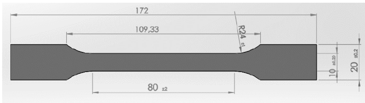
Figure 1. The dimensions of tensile test samples
