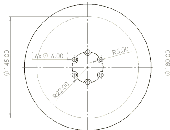
Figure 1. Bicycle disc brake rotor
