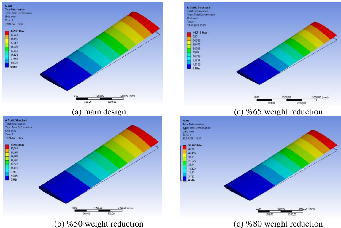
Figure 5. Total deformation values as a result of ANSYS structural analysis
