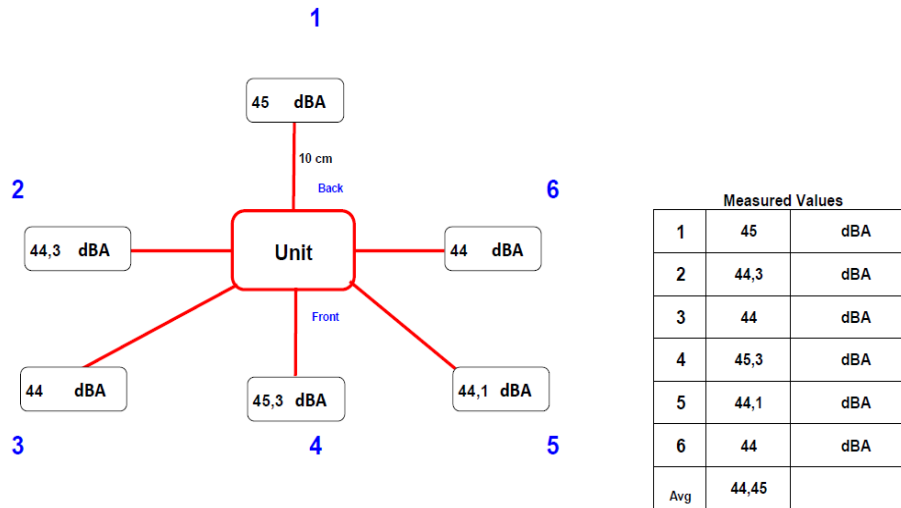
Figure 9: SLS Sound-Noise Level Test
