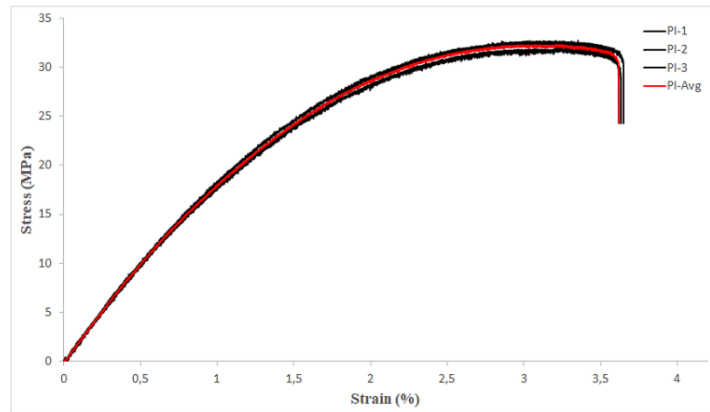
Figure 4: PI Tensile Stress- Strain Graph
