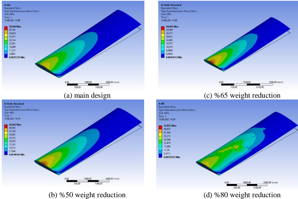
Figure 4. Von Mises stress values as a result of Ansys structural analysis
