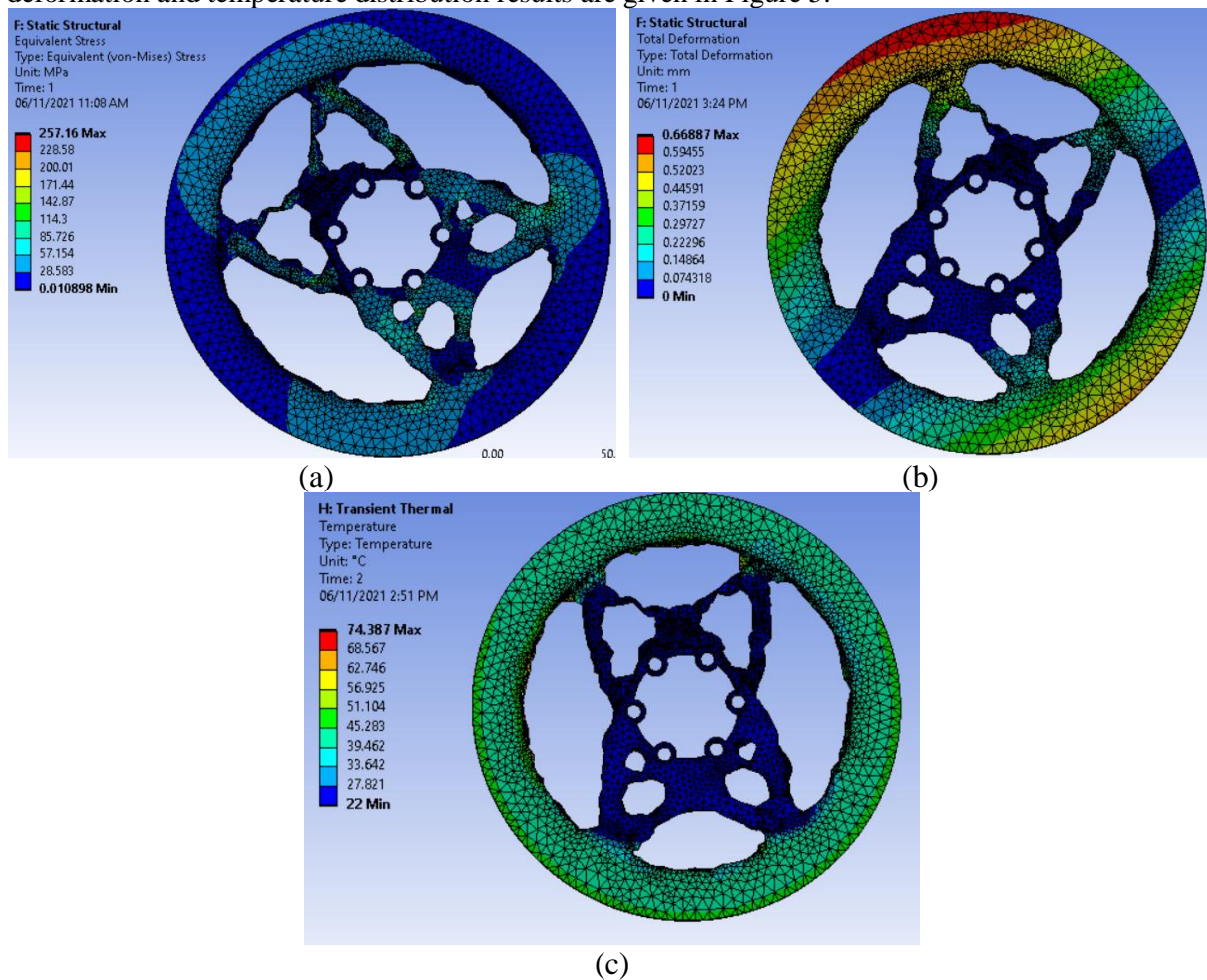
Figure 5. Rotor after topological optimization (a) Von-Mises stress (MPa) (b) total deformation (mm) (c) temperature distribution(°C)
