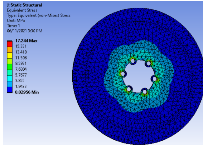
Figure 2. Rotor Von-Mises stress sistribution (MPa) before topological optimization
