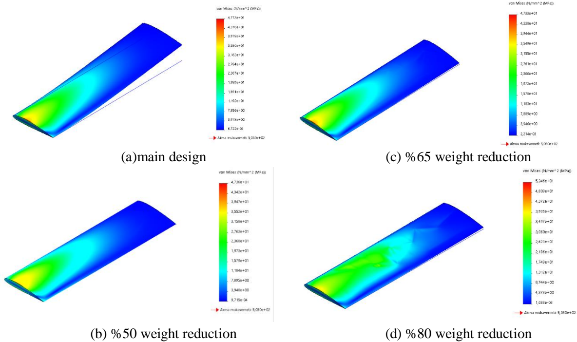
Figure 2. Von Mises stress values as a result of Solidworks structural analysis
