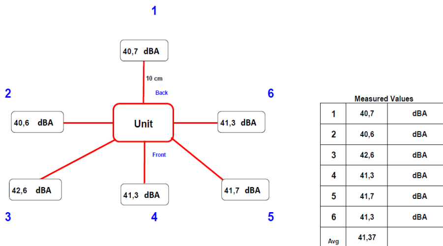
Figure 7: PI Sound-Noise Level Test
